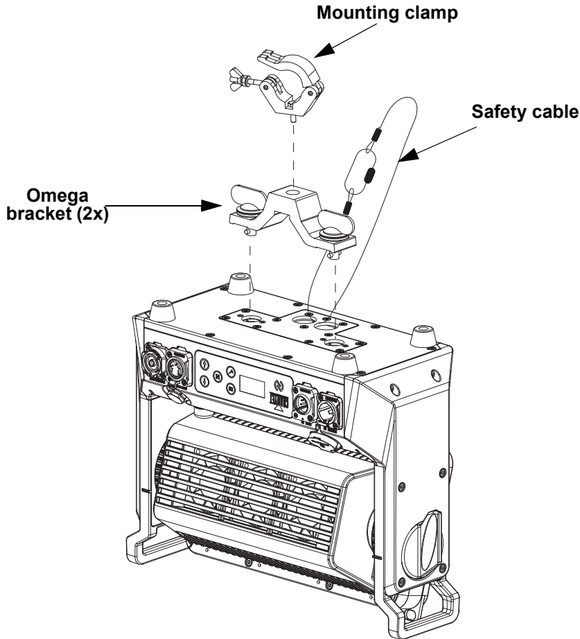
Overhead mounting
