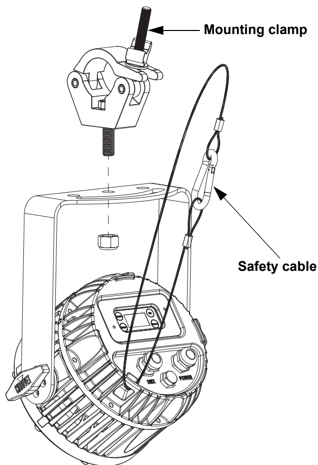
Overhead mounting
