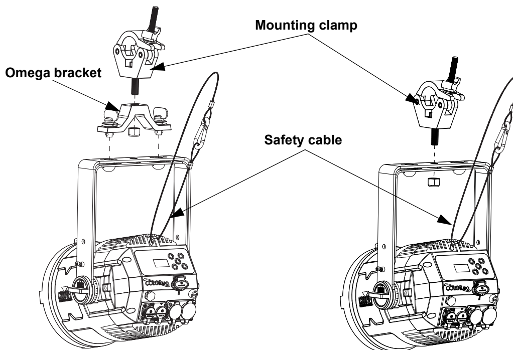
Overhead mounting
