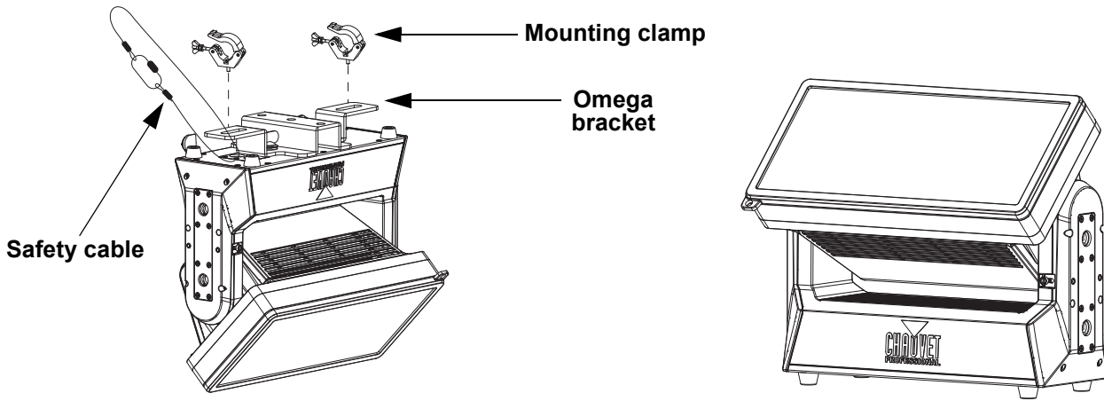
Overhead mounting
